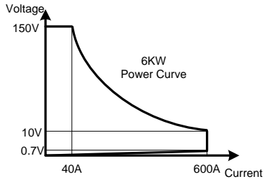
PEL-5006C-150-600 power contour
