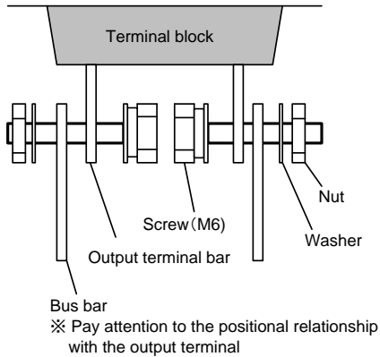
Parallel connection kit for vertical installation PSB-004
