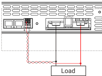
Sensor Wire Connections for 1U units
