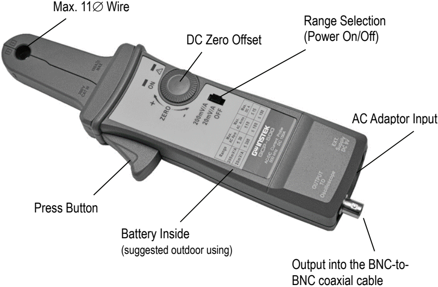
Figure 1. Shows the controls and indicators on the GCP-500 current probe.
